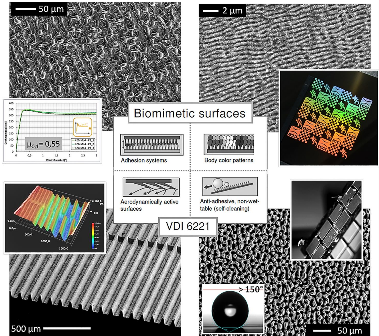
Skin friction drag reduction (Riblet)
